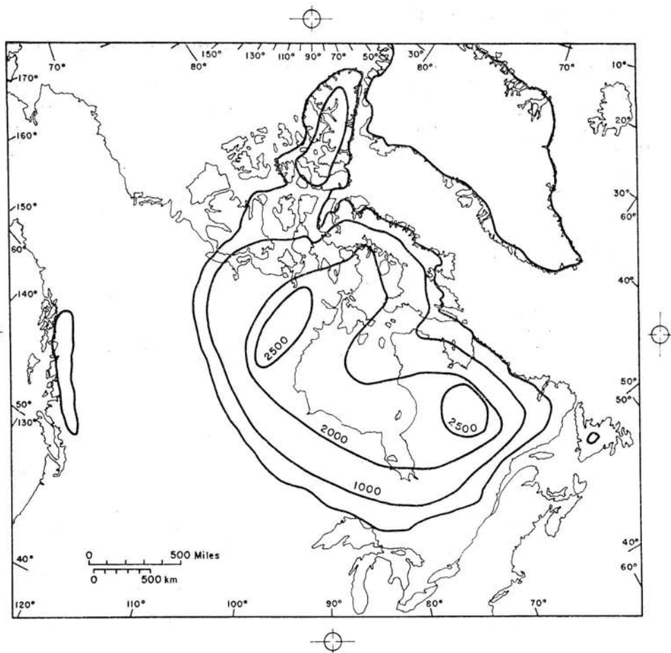
FIG. 9. Map of Laurentide ice thickness at 10 KYBP. Note the assumed splitting of the sheet into two main centres on either side of Hudson Bay by this time.
