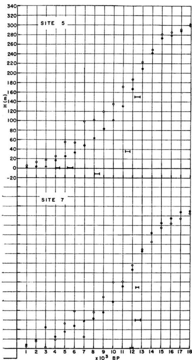
FIG. 13. Relaxation data at sites 4-7 compared with theoretical predictions from viscosity Models 1 and 3. Site numbers as shown.
