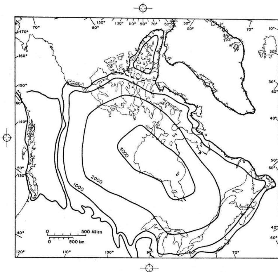
FIG. 8. Map of Laurentide ice thickness at the Wisconsin maximum approximately 18 KYBP. The Cordilleran, Innuitian, and Greenland sheets are also shown.
