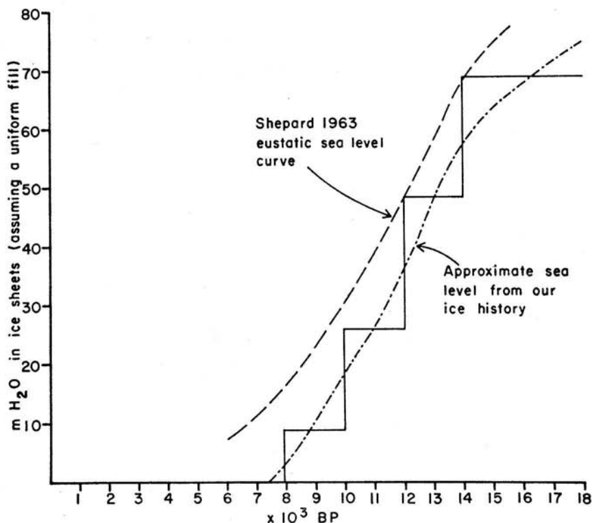
FIG. 10. Mean sea level history for ICE-1 contrasted with Shepard's (1963) generalized eustatic curve.
